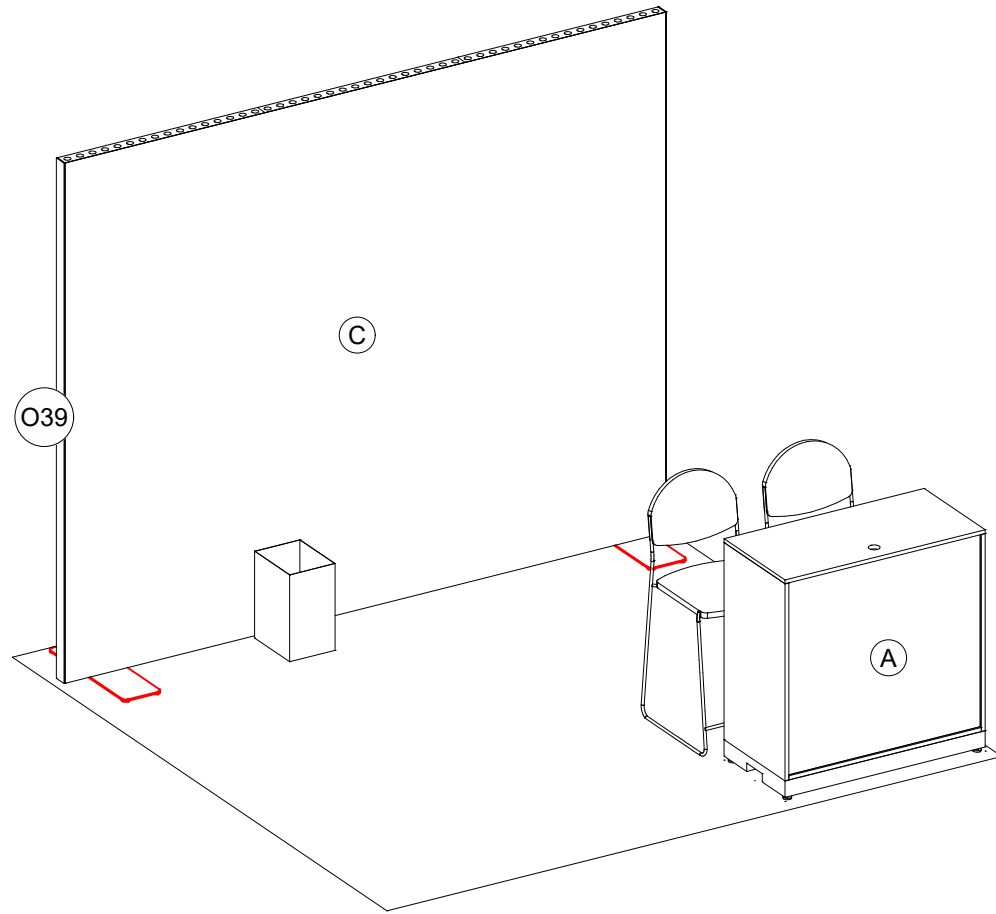
3D VIEW - 1
