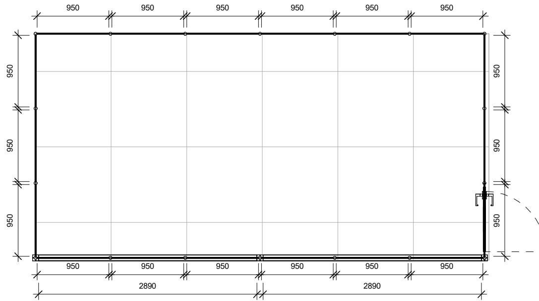
1 TOP VIEW 1 : 30
