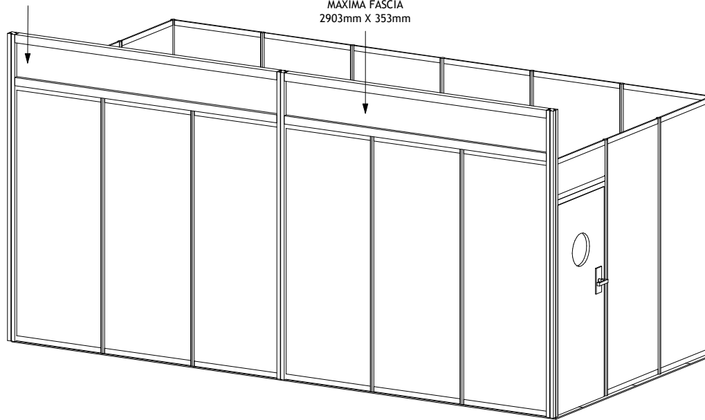
① ISOMETRIC VIEW
