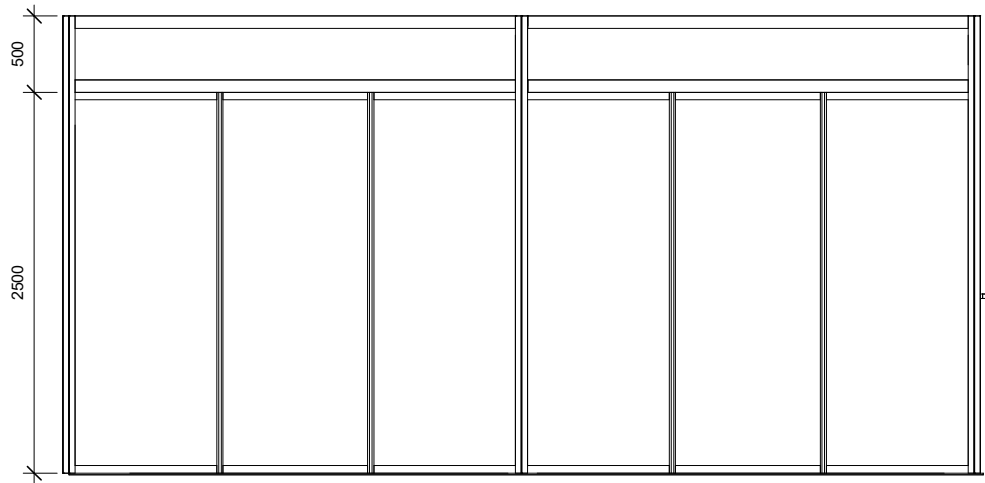
1 FRONT ELEVATION 1 : 30
