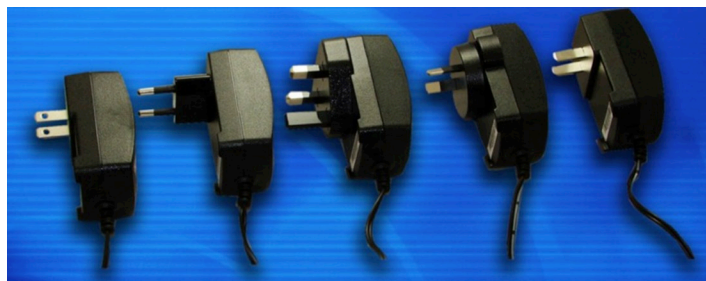
4-9. Phihong's energy-efficient 10W wall-mount adapter series is available in 5- and 9VDC outputs. The PSC12x Series consists of five versions: A, E, K, S, and C, each of which features a country-specific fixed-outlet plug. PSC12A adapters are equipped for use in the United States, Europe, United Kingdom, Australia, New Zealand, and China. PSC12x Series adapters are rated for operation from 0^{\circ}\text{C} to +40^{\circ}\text{C} .
