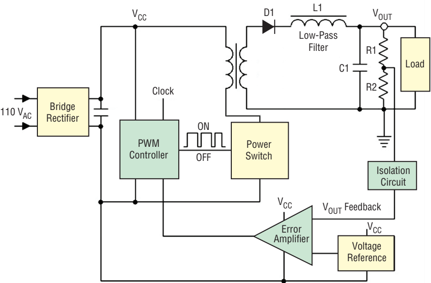
Figure 1-2. Typical Isolated AC-DC Switch- Mode Power Supply
